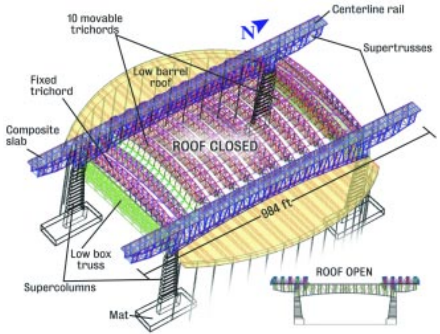
Schematic drawing of Reliant Stadium roof structure. The roof system was extensively tested to withstand wind uplift, unbalanced loading, lightning strikes and corrosion damage. It is the first roof of its kind to be constructed in the United States. The tri-chord-truss-framed roof splits and glides toward end zones on supertrusses.
